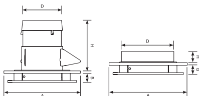
BDOP 80, 100, 125
