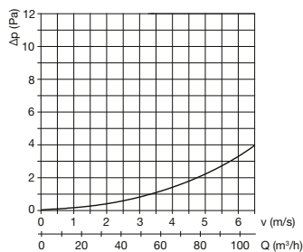
ED Flex® 90/75 EASY for 1 m of straight pipe
