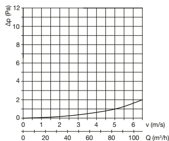
ED Flex® 90/77 PRO for 1 m of straight pipe
