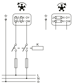
CMPB-Schaltplan
