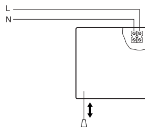
ECOAIR Design Ecowatt – M
