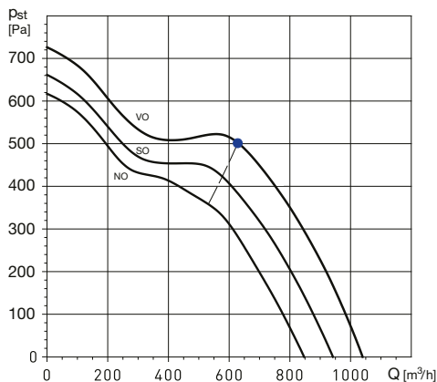
TDx2-800/200
