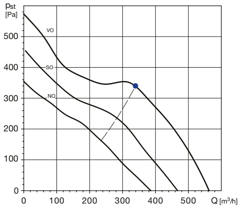
TDx2-500/150, TDx2-500/160
