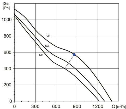
TDx2-1300/250
